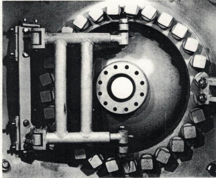
Fig. 2.14. Double-hinged one-way pressure door.
